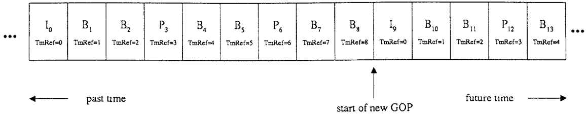
Video Stream in Display Order
